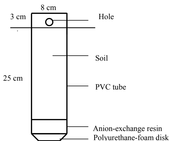
Figure 2.10: Equipment for in situ studies of N-mineralization
