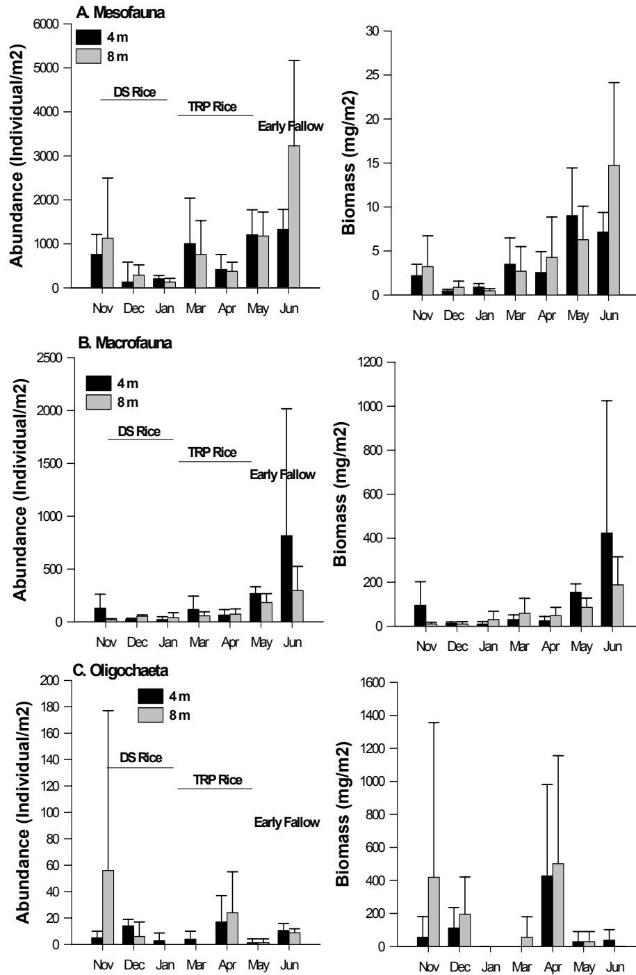
Figure 3.8: The effect of 4-m and 8-m bund distances on soil fauna abundance and biomass in dry-seeded rice (DS Rice), transplanted rice (TRP Rice) and early fallow (soil depth 0-15 cm; ANOVA on log- transformed fauna data; *: P < 0.05 , **: P < 0.01 )
