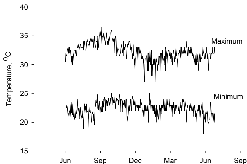
Figure 2.4: Daily minimum and maximum air temperatures at Jakenan Research Station, Pati, Indonesia, during the study period from June 2000 to June 2001.
