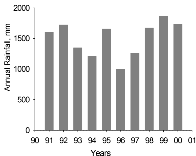
Figure 2.2: Annual rainfall in Pati District, for the period of 1991 to 2000.
