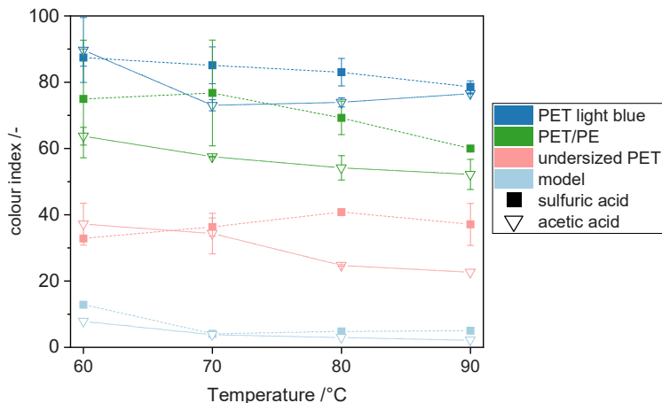
Figure 5-11 Hazen colour index of TA precipitated with sulfuric and acetic acid at various temperatures, single measurements for model reactant only, lines are shown to guide the eye. 102
