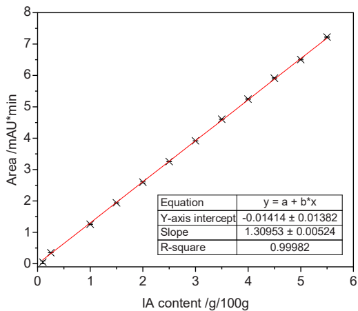
Figure 8-4 Linear fit of chromatogram area (mAU*min) over IA content for determination of IA content in rTA.
