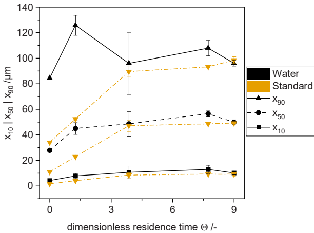
Figure 8-15 x_{3,10} , x_{3,50} and x_{3,90} quantiles of TA after precipitation with sulfuric acid at 80 °C with different initial reactor content, lines are shown to guide the eye.
