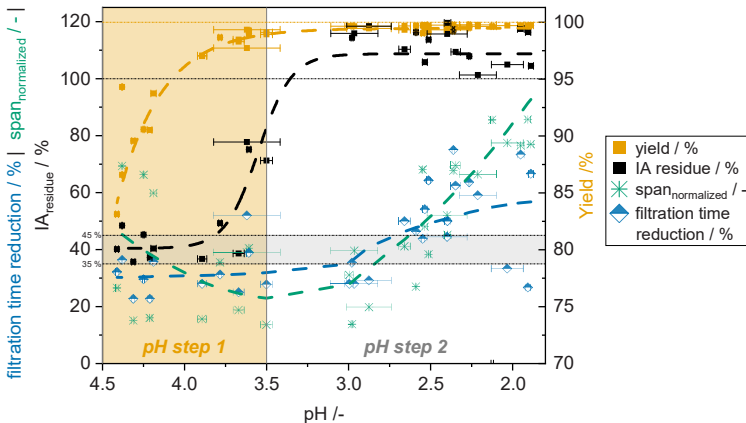
Figure 6-15 Yield, IA residue, normalized span and filtration time reduction of TA after precipitation at 80 °C with sulfuric acid over respective pH, all values refer to pH at t_{3,87} and t_9 according to Figure 8-20, lines are shown to guide the eye.
