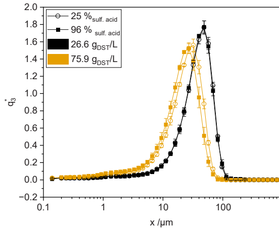
Figure 8-9 PSD of TA after precipitation at 80 °C in PET light blue reactant of different concentrations, t_0 samples.
