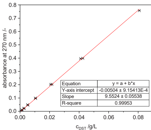
Figure 8-3 Linear fit of absorbance at 270 nm over DST concentration for determination of initial and residual DST content.
