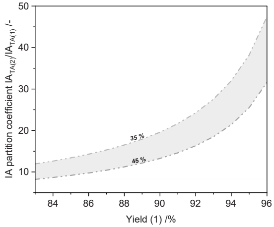
Figure 8-21 Partition coefficient of IA content between TA(1) and TA(2) over yield of the first precipitation step.
