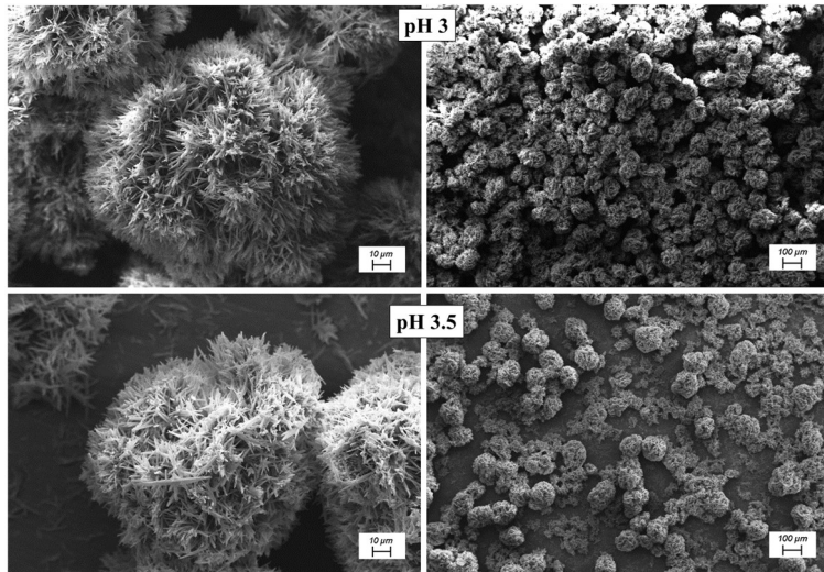
Figure 6-14 SEM images of rounded TA morphology after precipitation with sulfuric acid at 80 °C at constant pH of 3 (75.9 g DST /L) and 3.5 (26.6 g DST /L), left images show 500 x and right 50 x magnification.
