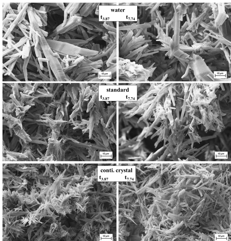
Figure 8-17 SEM images of TA from for PET/PE reactant after precipitation at pH 3.5 with sulfuric acid at 80 °C, start-up variation, t_{3.87} (left) and t_{7.74} (right).
