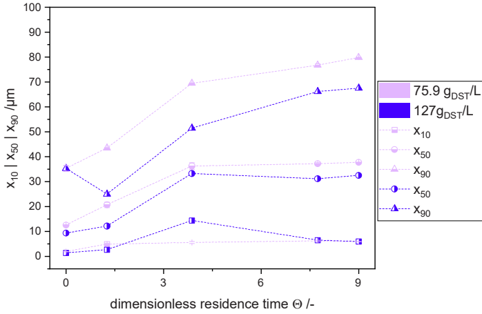
Figure 8-10 Quantile Values of TA after precipitation with 25 % sulfuric acid at 80 °C in PET/PE reactant of different concentrations.
