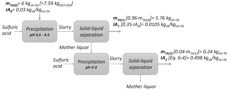
Figure 6-17 Block flow diagram of two-step precipitation concept with mass balance example for a PET reactant with an initial IA_0 of 3%.
