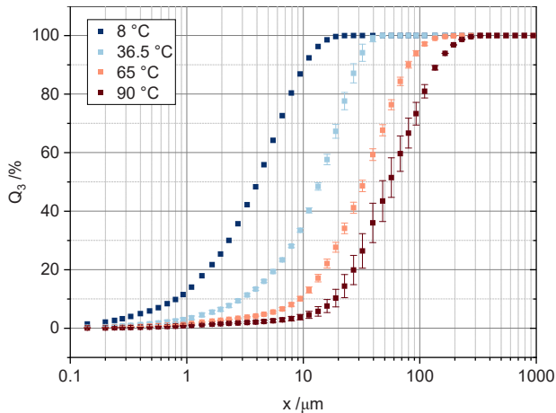
Figure 5-2 Volume-related cumulative PSD of TA after precipitation with acetic acid at different temperatures, 8 \text{ }^\circ\text{C} acetic acid represents single measurement only. 17
