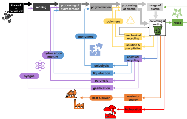
Figure 3-3 Simplified plastic lifecycle and classification of recycling technologies with regard to respective input and output streams, colour code from green to red refers to qualitative effort for plastic reapplication, adapted from Brepohl et al.. 49
