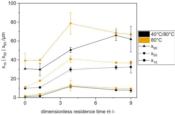
Figure 8-14 x_{3,10} , x_{3,50} and x_{3,90} quantiles of TA after precipitation with sulfuric acid with different initial precipitation temperatures, lines are shown to guide the eye.
