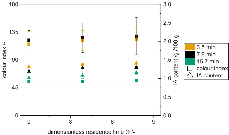
Figure 6-7 Colour index and IA content of TA after precipitation with sulfuric acid at 80 °C for different residence times
