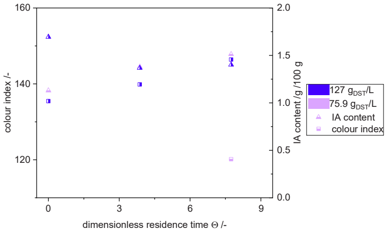
Figure 8-11 Purity of TA after precipitation with 25 % sulfuric acid at 80 °C in PET/PE reactant of different concentrations.
