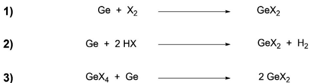
Schema 2. Synthese der Germaniumdihalogenide \text{GeX}_2 ( \text{X} = \text{F}, \text{Cl}, \text{Br}, \text{I} ).
