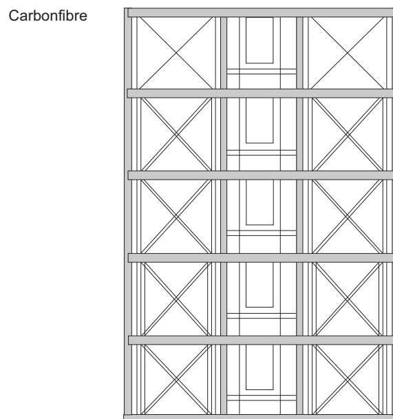
Figure 4.14: Layout of reinforcing carbon fibre on a RC building with masonry infill and five floors.
