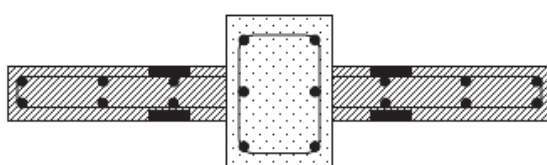
Figure 4.4: Detail of the reinforced concrete side wall type in horizontal section
