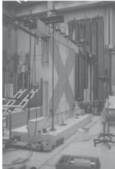
Figure 4.13: Experimental tests on masonry wall reinforced with glass fibre in the laboratory of the “Institute for Massivbau”
