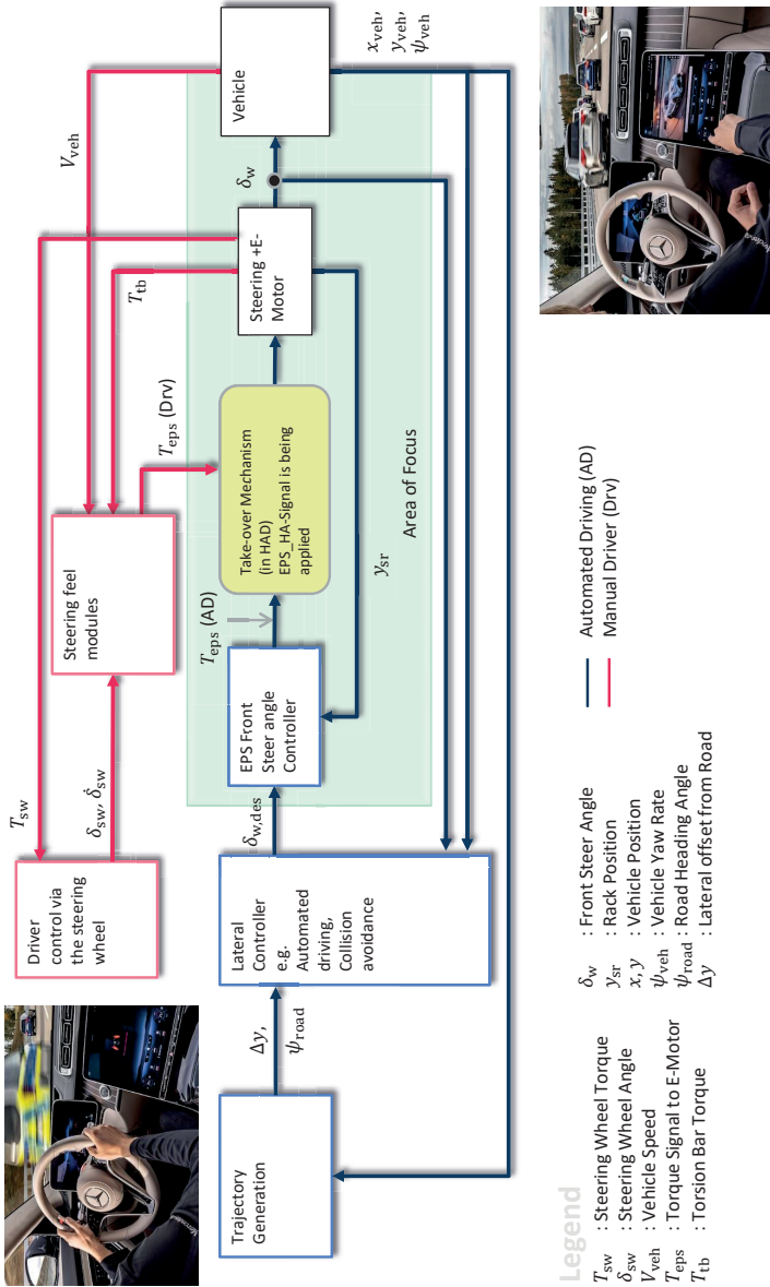
Figure 1.3: This figure shows the system's architectural paths for manual and autonomous driving
